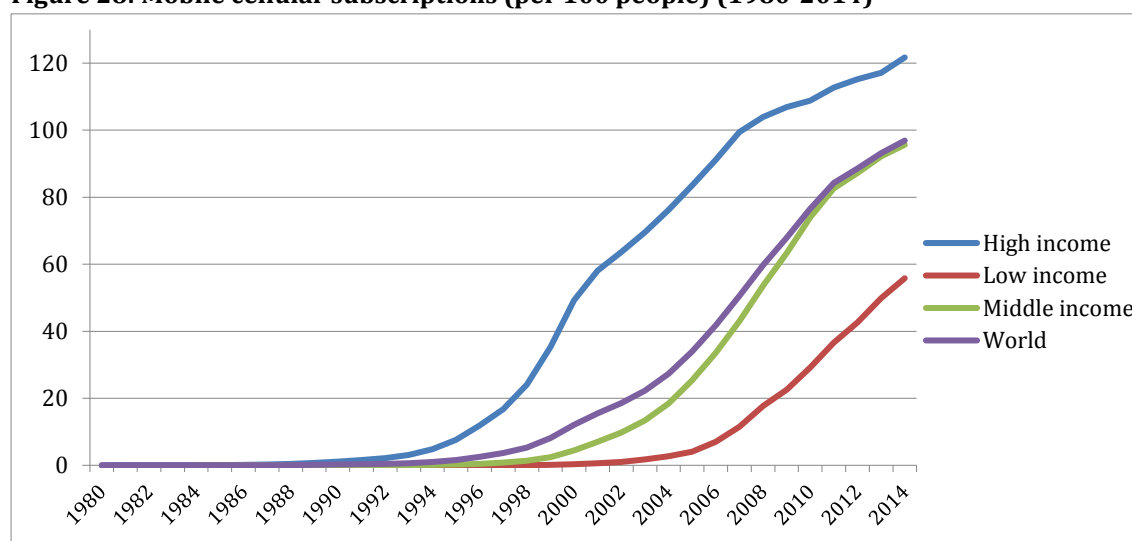
Figure 28: Mobile cellular subscriptions (per 100 people) (1980-2014)
